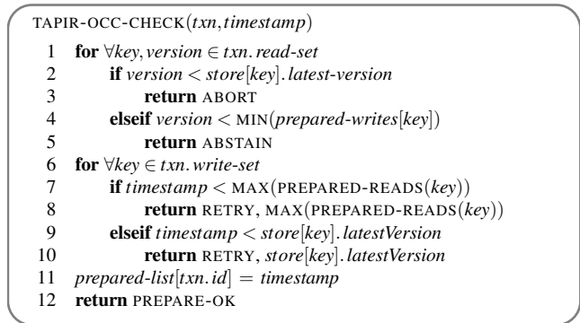
Figure 8: Validation function for checking for OCC conflicts on Prepare. PREPARED-READS and PREPARED-WRITES get the proposed timestamps for all transactions that the replica has prepared and read or write to key , respectively.
