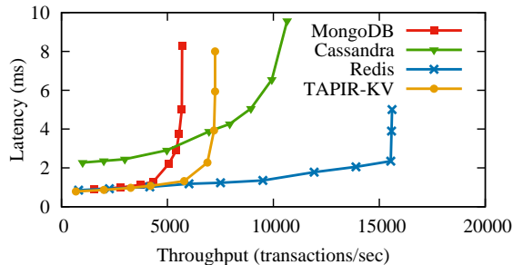
Figure 14: Comparison with weakly consistent storage systems.
