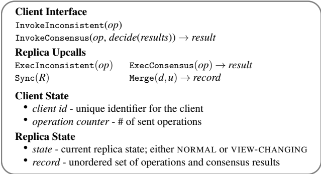
Figure 3: Summary of IR interfaces and client/replica state.
